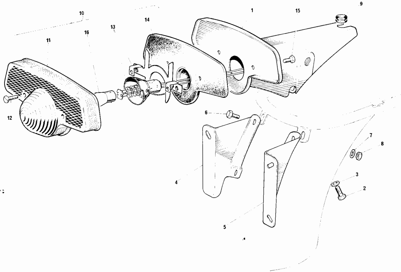
Fig. 25. TAIL LAMP AND SUPPORT
