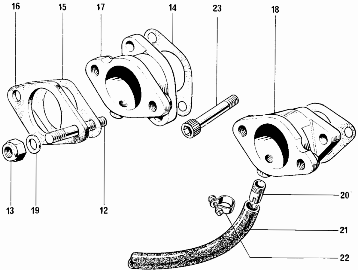
Fig. 4. INLET MANIFOLDS
