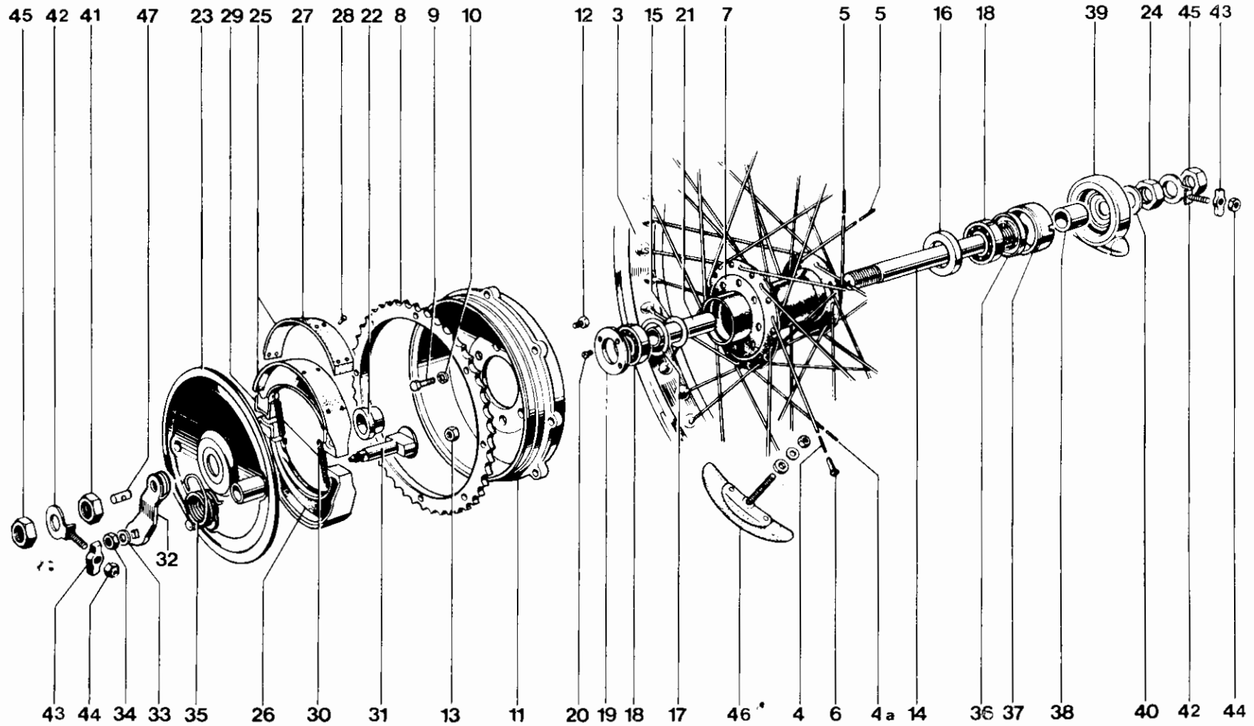
Fig. 32. REAR WHEEL
