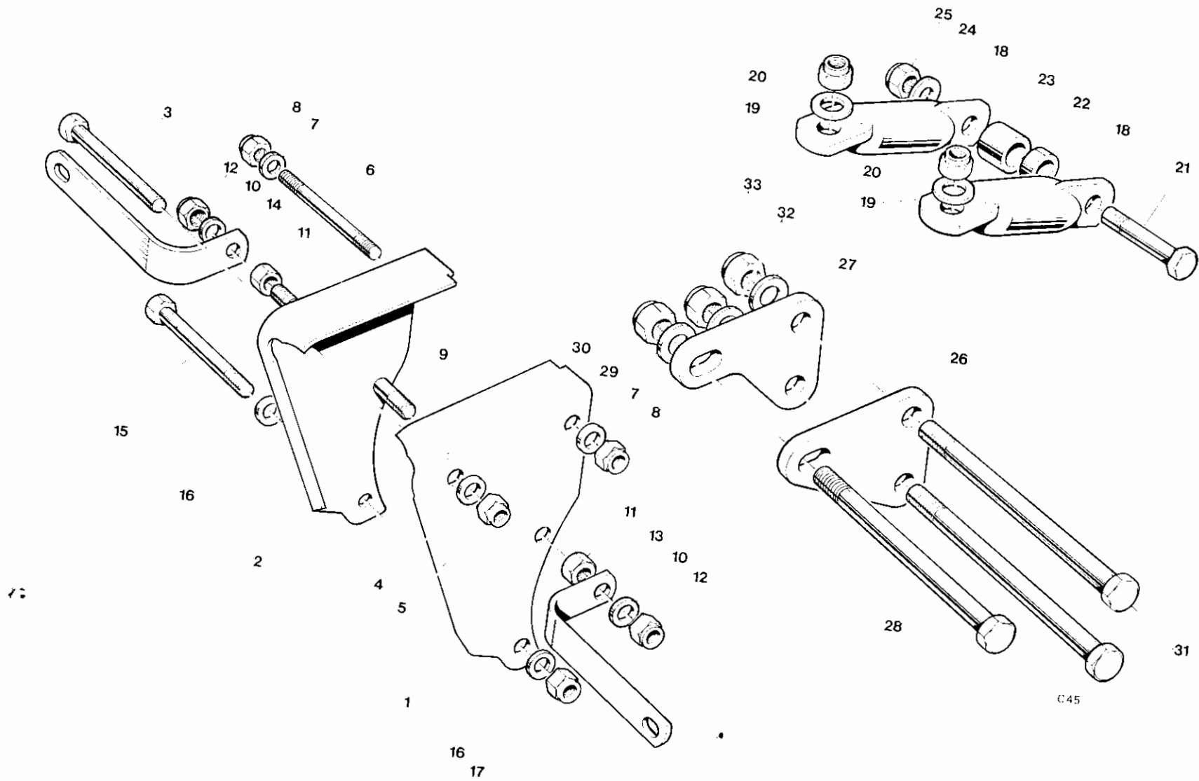
Fig. 16. MOTOR FITTINGS
